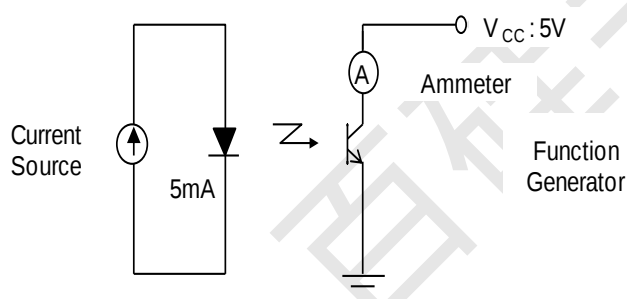
Fig 1. Test Circuit for I C
