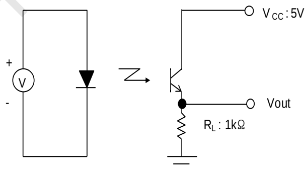
Fig 2. Test Circuit for Rise and Fall Time
